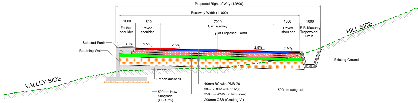
TYPICAL CROSS-SECTION OF ROAD IN ONE SIDE HILL AND ONE SIDE VALLEY
