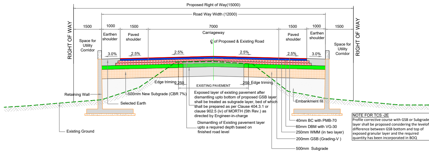
TYPICAL CROSS-SECTION OF ROAD WITH BOTHSIDE RETAINING WALL
