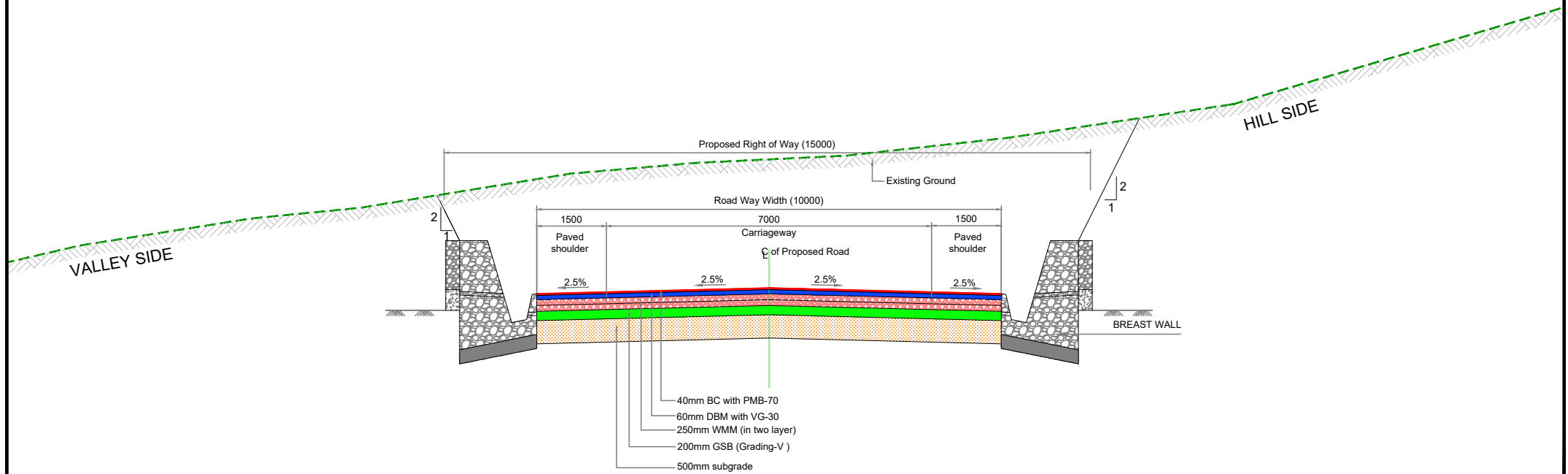
TYPICAL CROSS-SECTION OF ROAD IN HILL AREA
