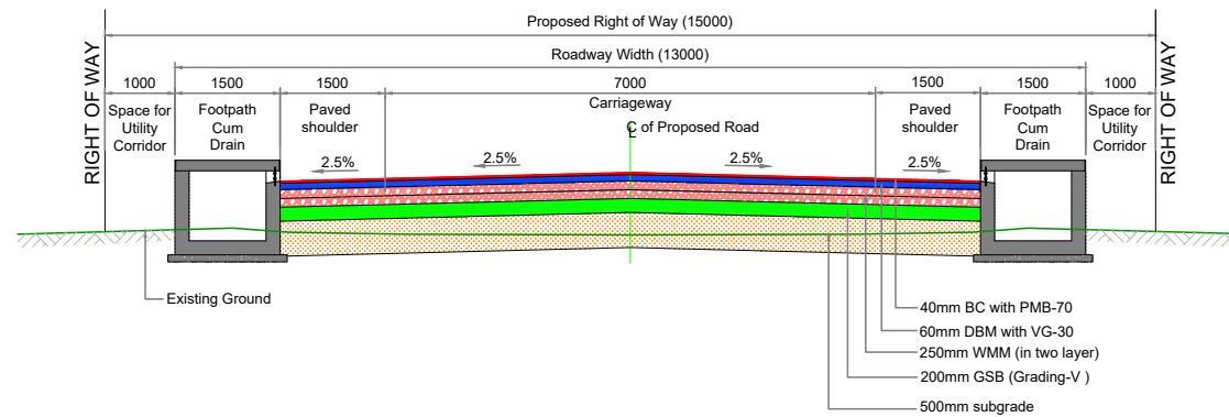
TYPICAL CROSS-SECTION OF ROAD IN BUILTUP AREA
