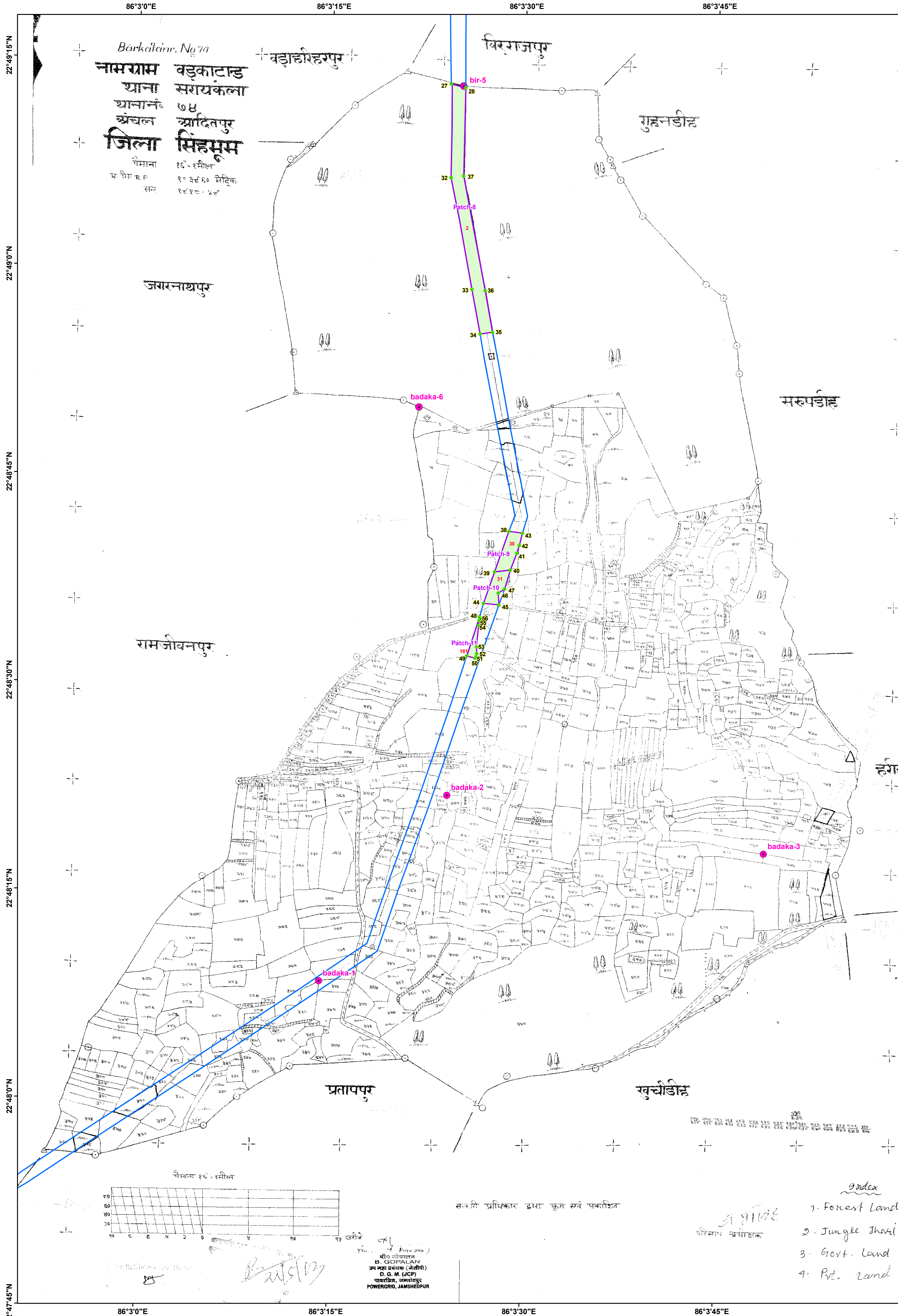
Map Showing DGPS Surveyed Co-ordinates and Boundary of Forest Land Proposed to be diverted for 220kV D/C Ramachandrapur - Chaibasa Transmission line under Village- Badakataand State:Jharkhand
