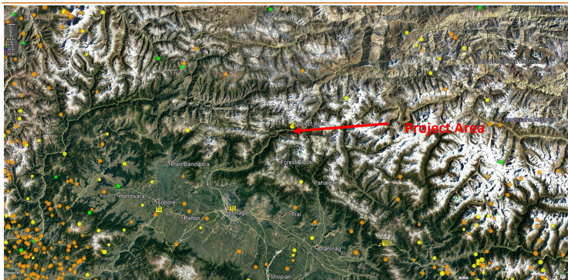
Fig6. 7-3: Major earthquake in the vicinity of the project area.
