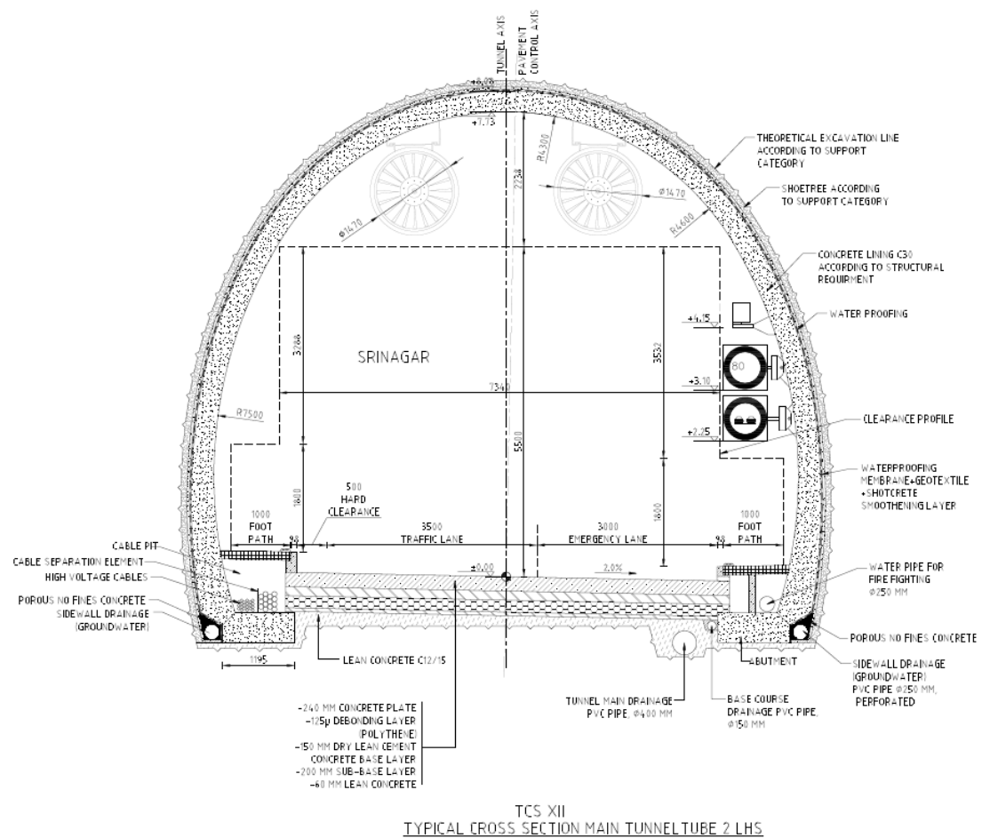
Fig. 7-2: Typical Section of Tunnel LHS Tube
