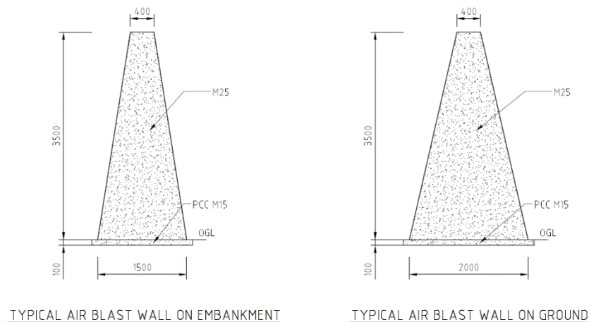
Fig. 6-27- Typical Section of Air Blast Wall
