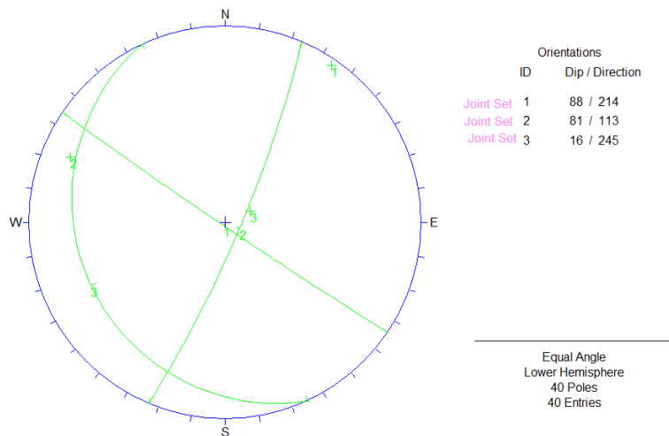
Fig. 6-20: Stereoplot of the Discontinuities
