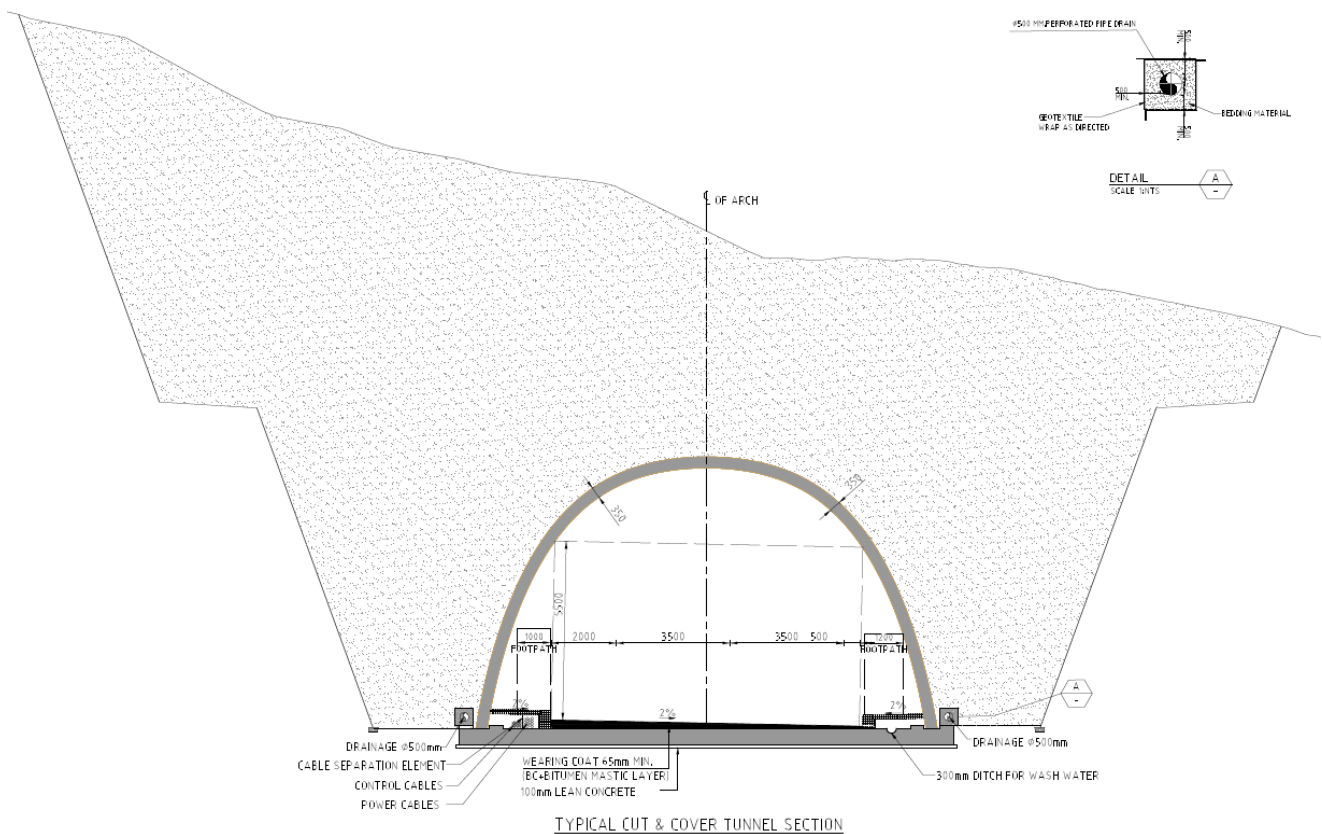
Fig. 7-3: Typical Cut & Cover Section
