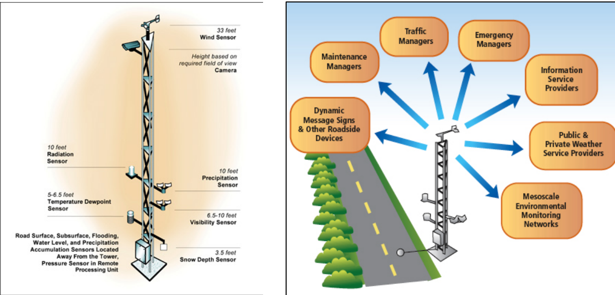
Fig. 12-3 : Environmental Sensing Stations
