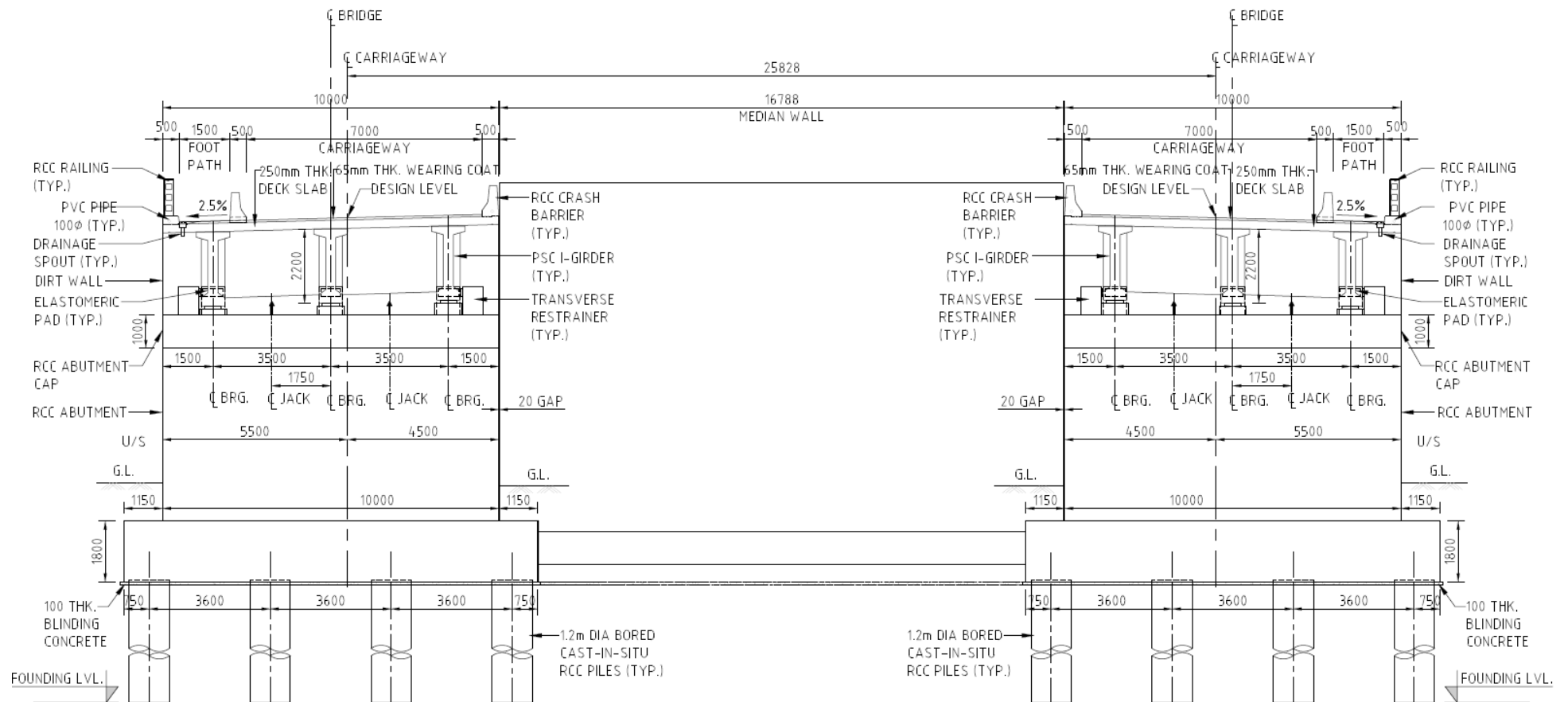
TCS TYPE XIA TYPICAL CROSS-SECTION OF BRIDGE WITH PROTECTED FOOTPATH AS PER IRC-SP-73-2015
