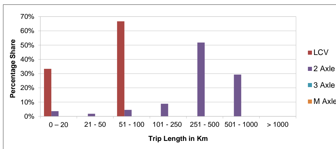
Fig. 4-23: Trip length distribution of Commercial Vehicles at Km – 85+800
