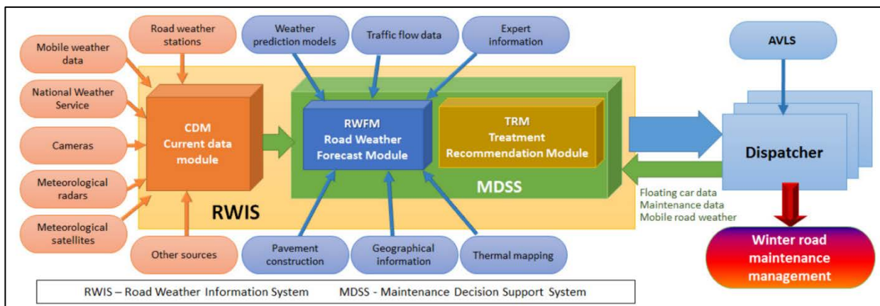
Fig. 12-2: The basic components and scheme of intelligent winter road maintenance management
