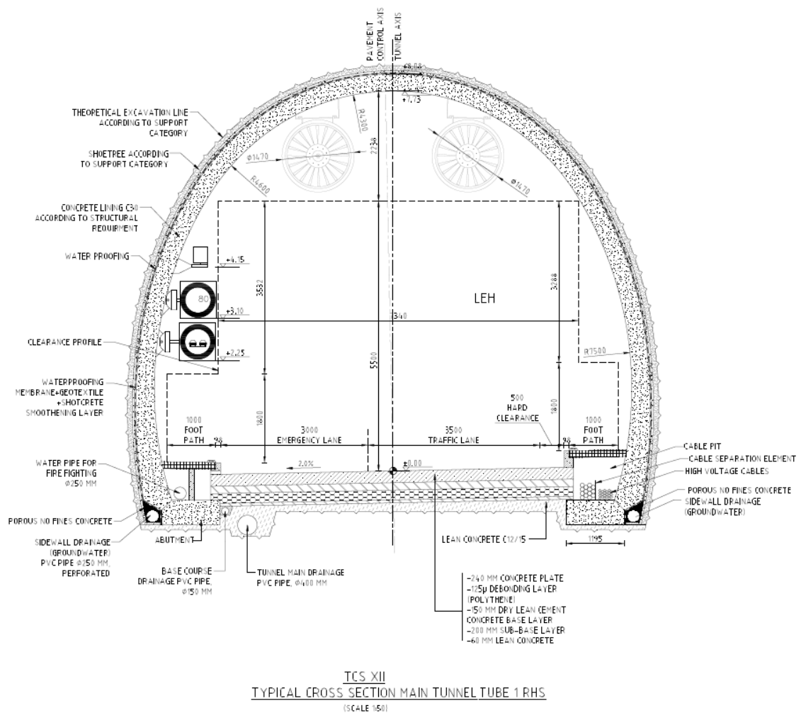
Fig. 7-1: Typical Section of Tunnel RHS Tube
