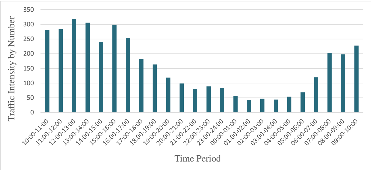
Fig. 4-6: Hourly Variation Traffic at Km- 85+900
