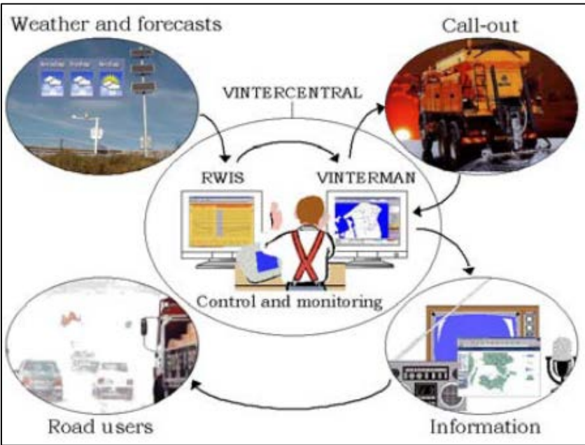
Fig. 12-1: RWIS – Road weather information system (Source: Snow and ice data book 2006)
