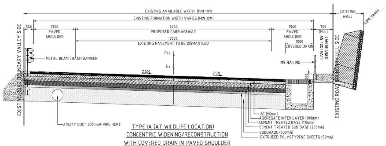
Figure 1-2 Proposed Road Configuration at Wildlife location
