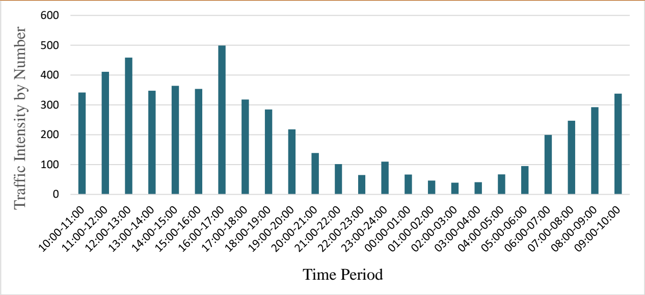
Fig. 4-5: Hourly Variation Traffic at Km- 81+600
