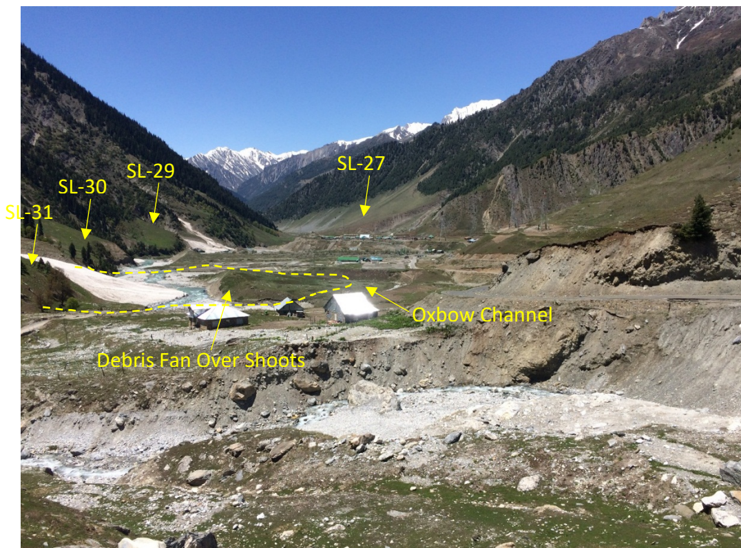
Fig. 6-10 : SL-29 to 31/ left bank debris fans extending beyond river (cut through by river/ that of 31 has an Oxbow)
