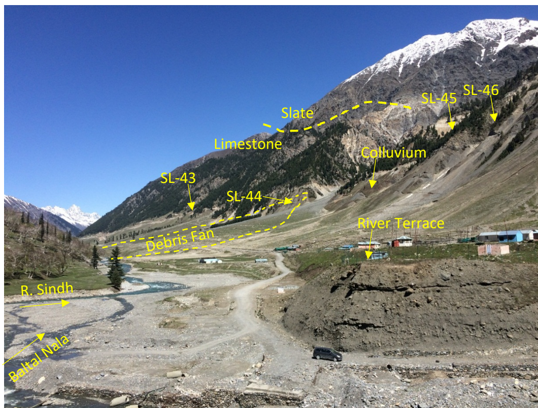
Fig. 6-9: Sindh River low terraces and debris fans (SL-44 in main)
