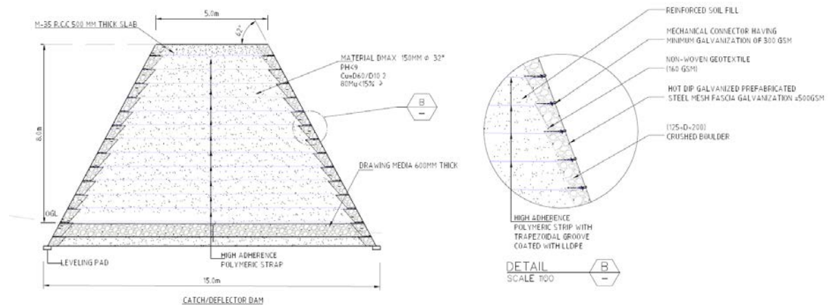
Fig. 6-26- Typical Section of Catch/Deflection Dams
