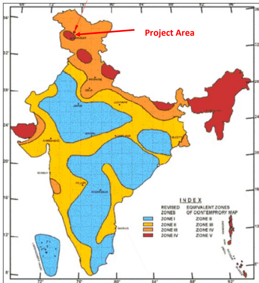
Fig. 6-2: Project located in Zone-V as per seismic zoning map of India.
