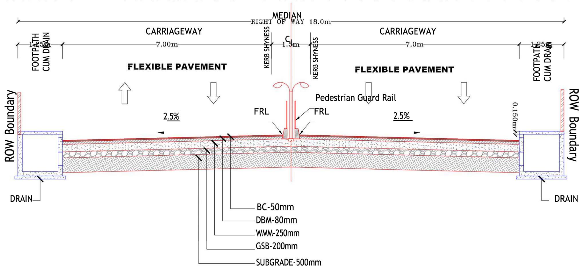
TYPICAL CROSS SECTION : TYPE-1
