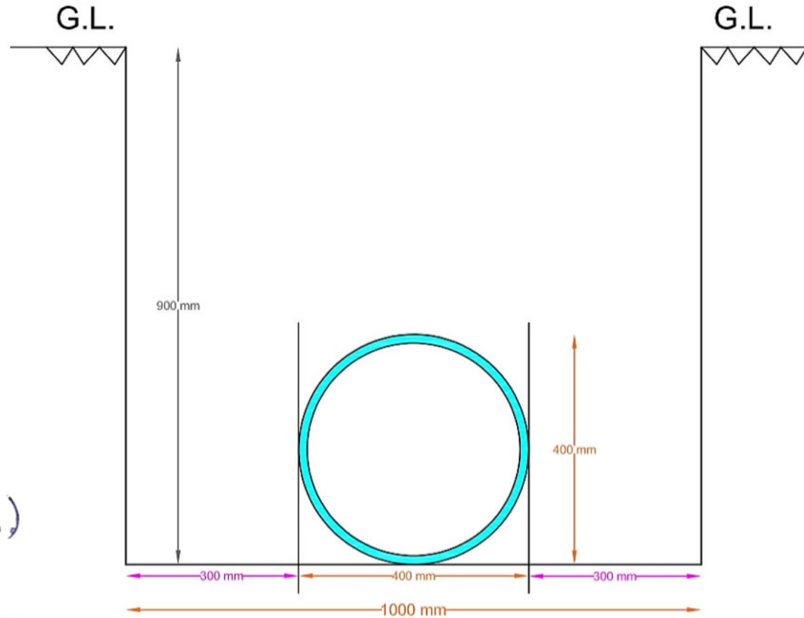
TYPICAL CROSS SECTION FOR LAYING OF 400 MM PIPELINE (1.00 Metere RoW)
