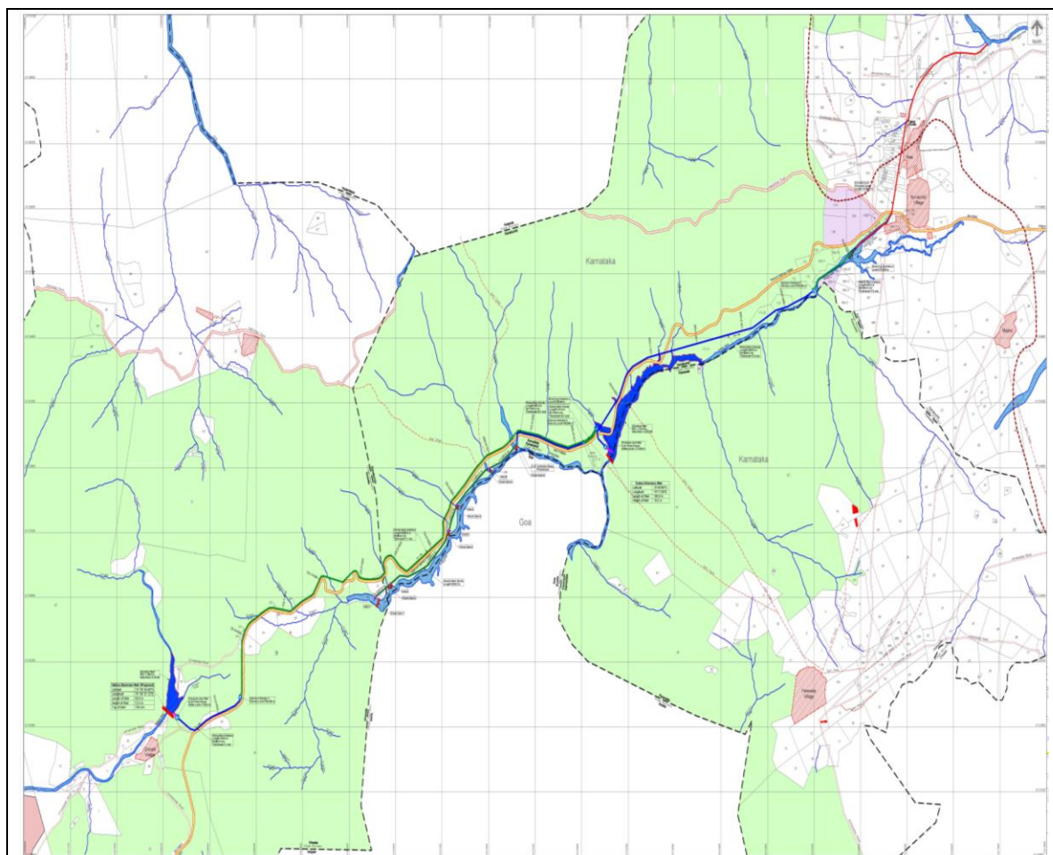
Figure 1: Master Plan of Kalasa Diversion Scheme.
