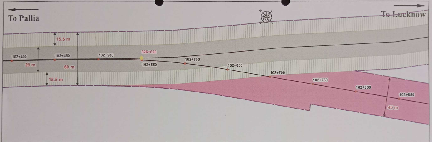
Strip Map/Linear Plan Improvement and Up-gradation of Existing Road (NH-731) to 4-Lane with Paved Shoulder from Km 88.750 to Km 123.650, Start of Shahjahanpur Bypass to Start of Shahabad Bypass of NH-731 on HAM basis of Shahjahanpur and Hardoi Forest Division, Shahjahanpur and Hardoi District in the state of Uttar Pradesh (Total Length-34.900 Km of Package 2A)
