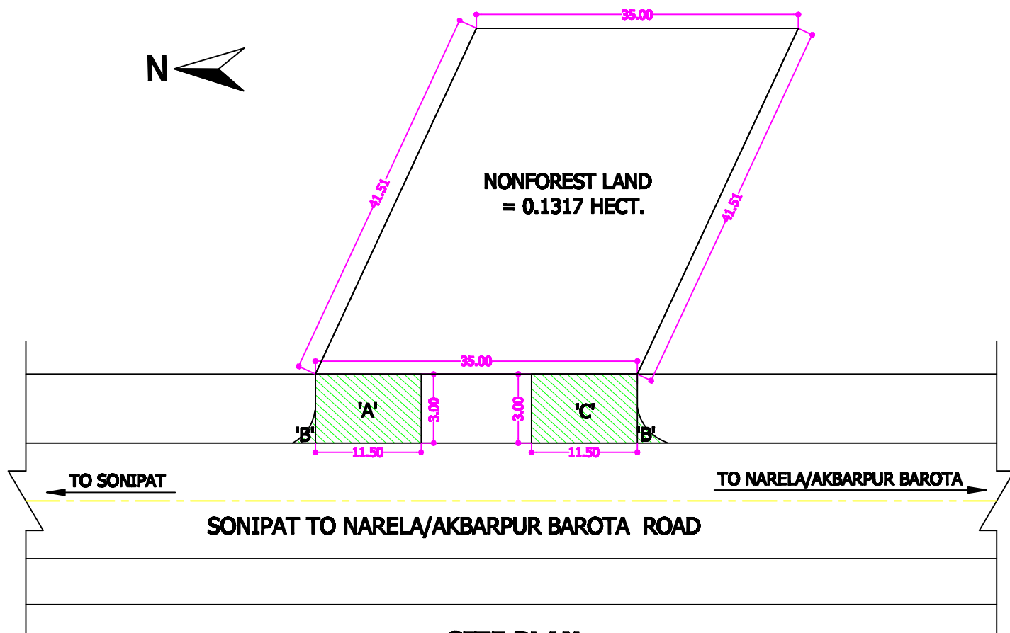
SITE PLAN
