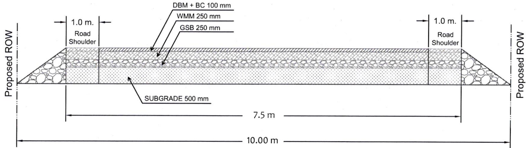
TYPICAL CROSS SECTION (Inside the Forest Land)
