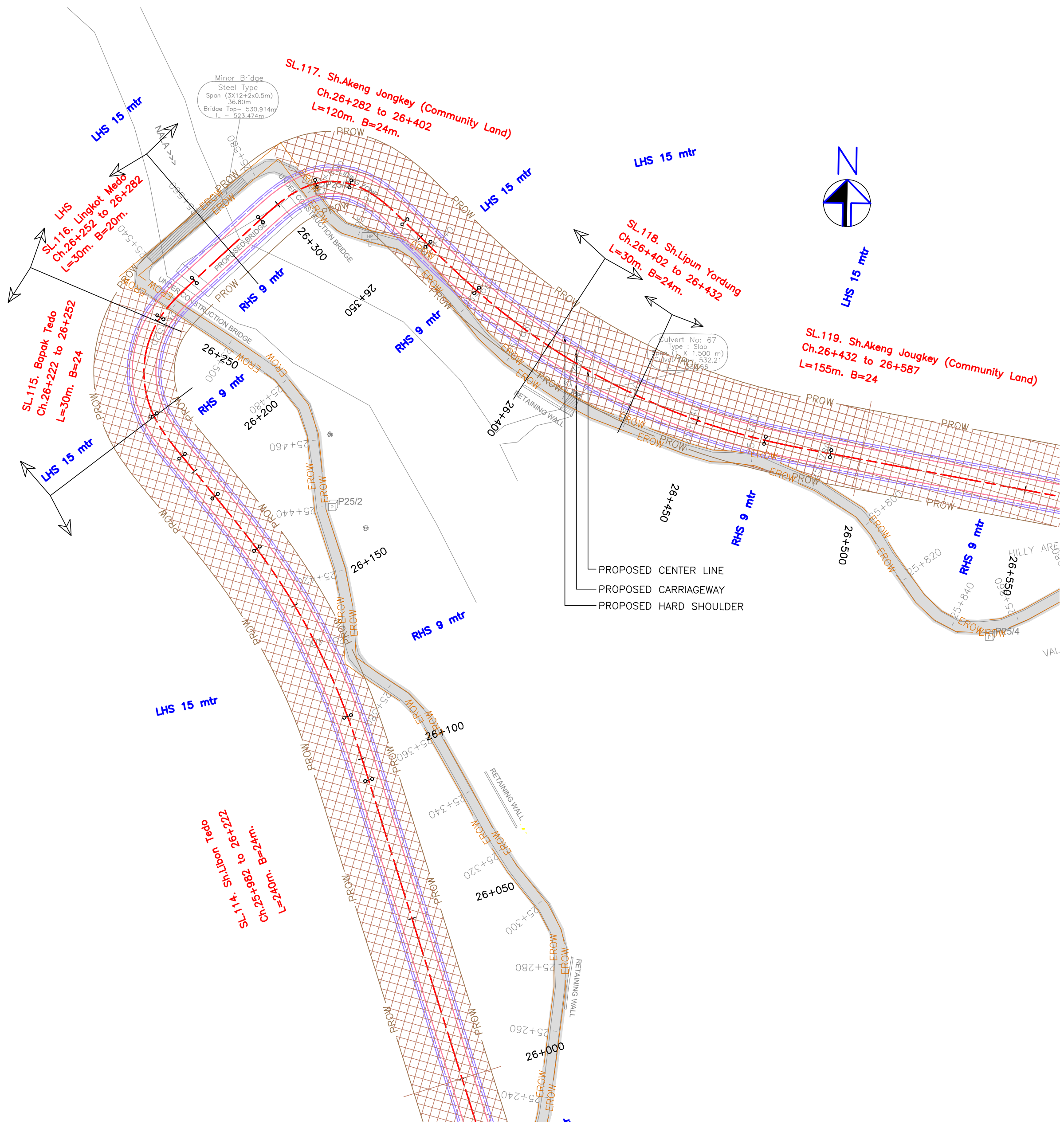
PLAN-KM 26+000 TO KM 26+500
