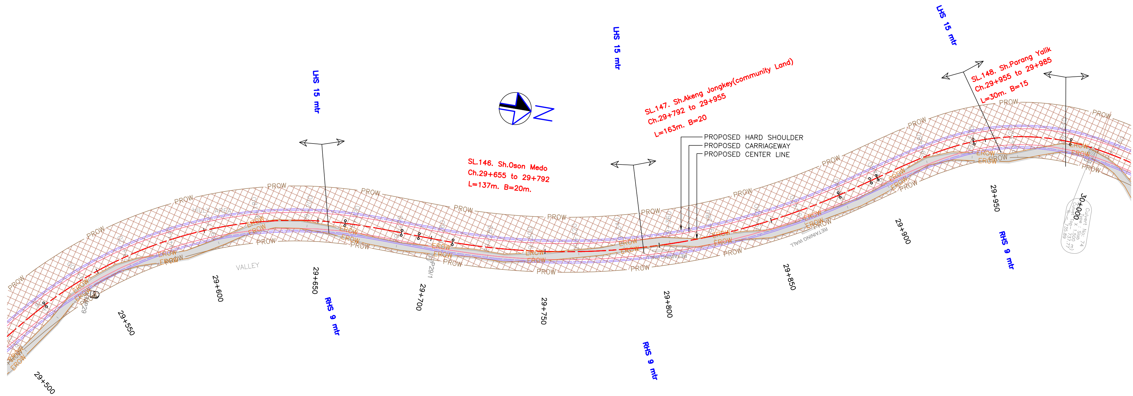
PLAN-KM 29+500 TO KM 30+000
