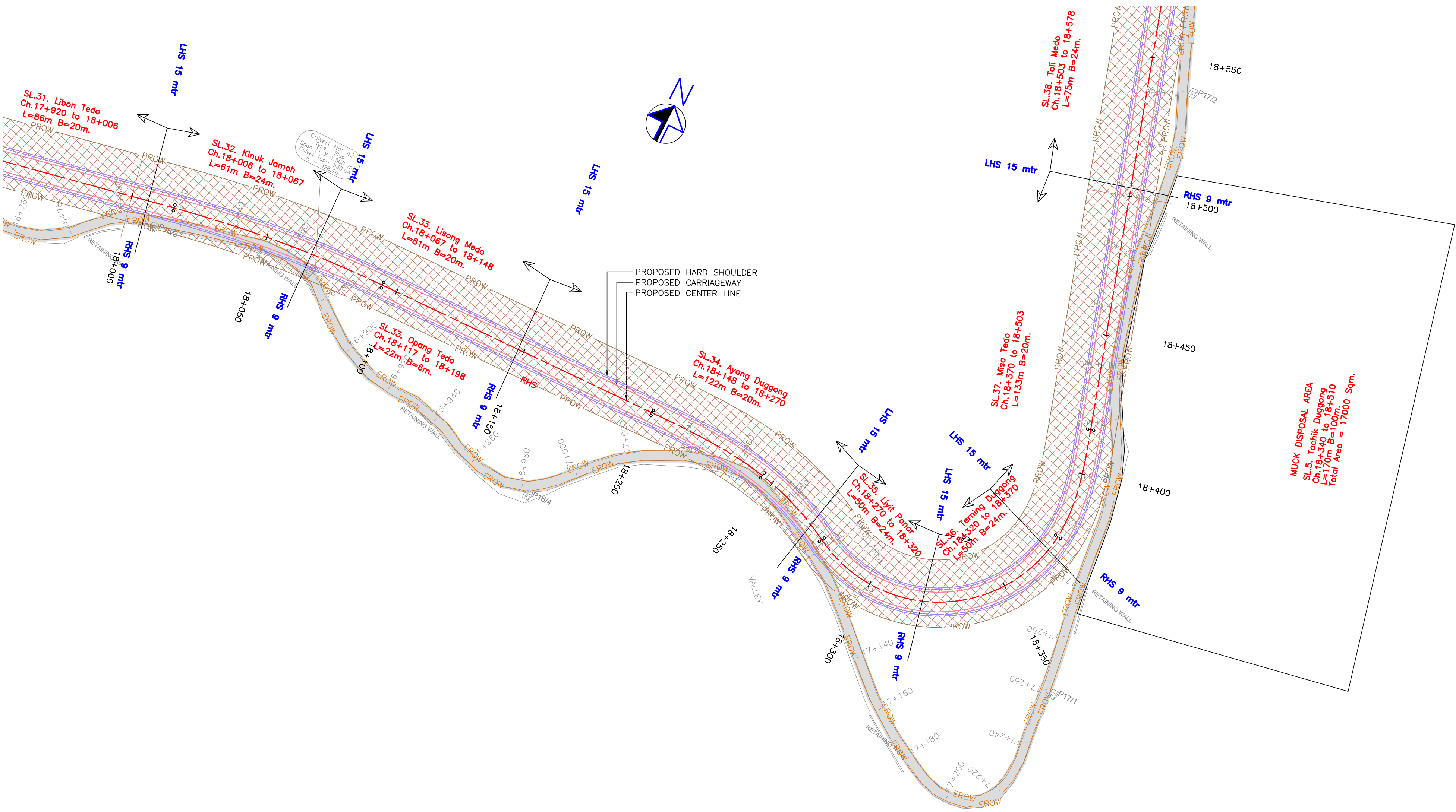
PLAN-KM 18+000 TO KM 18+500
