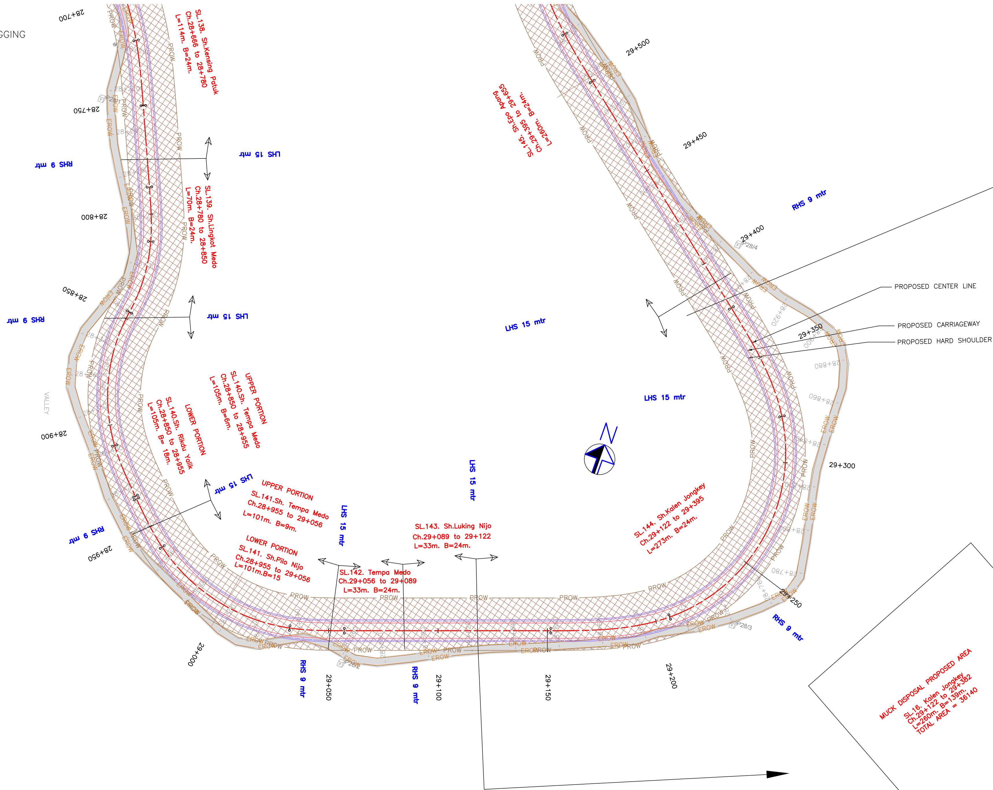
PLAN-KM 29+000 TO KM 29+500
