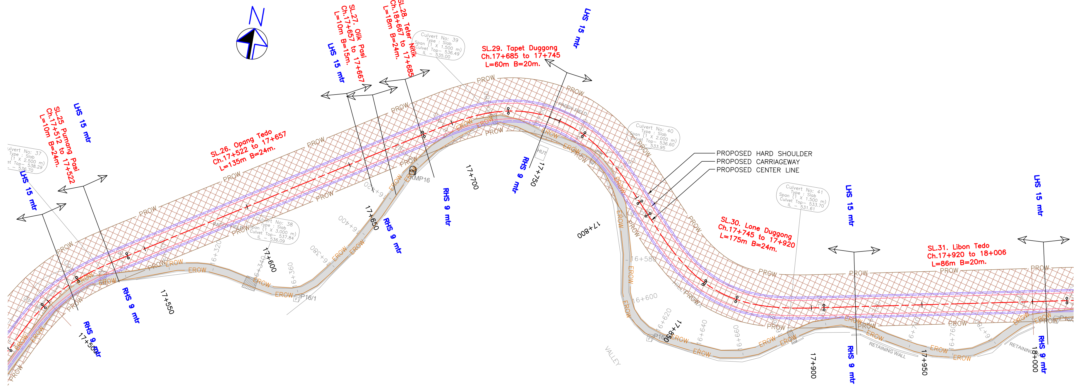
PLAN-KM 17+500 TO KM 18+000
