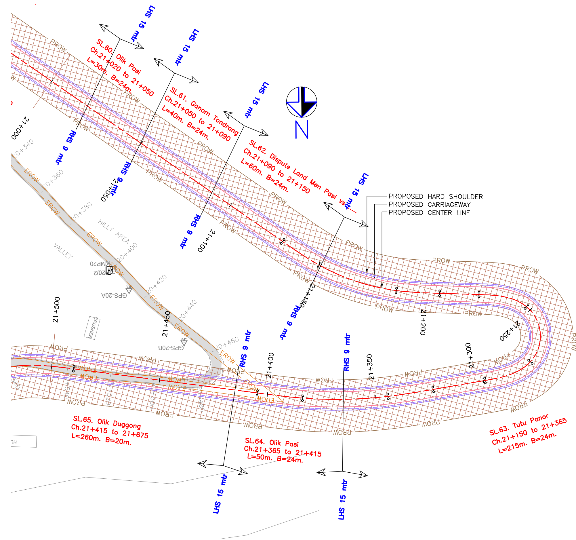
PLAN-KM 21+000 TO KM 21+500
