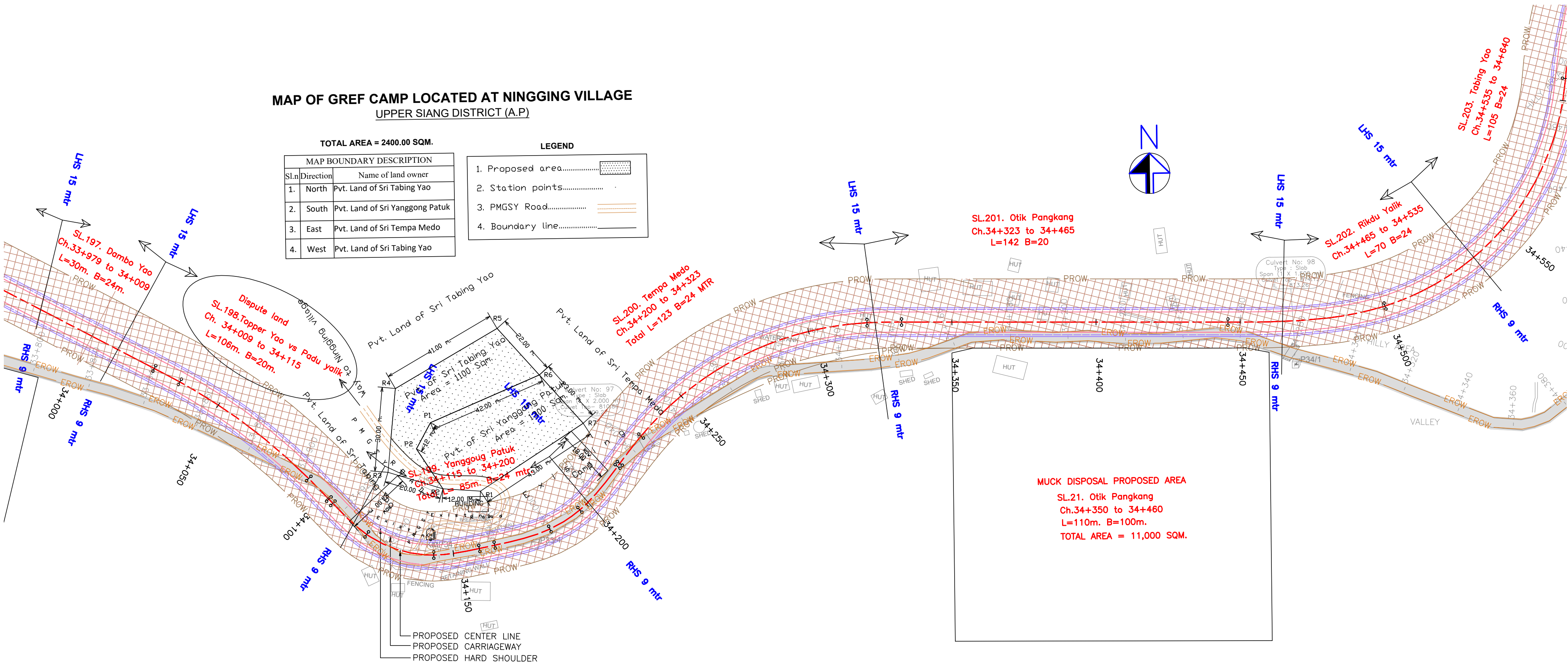
PLAN-KM 34+000 TO KM 34+500
