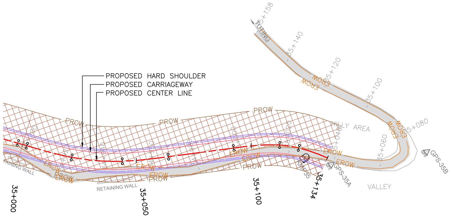
PLAN-KM 35+000 TO KM 35+134
