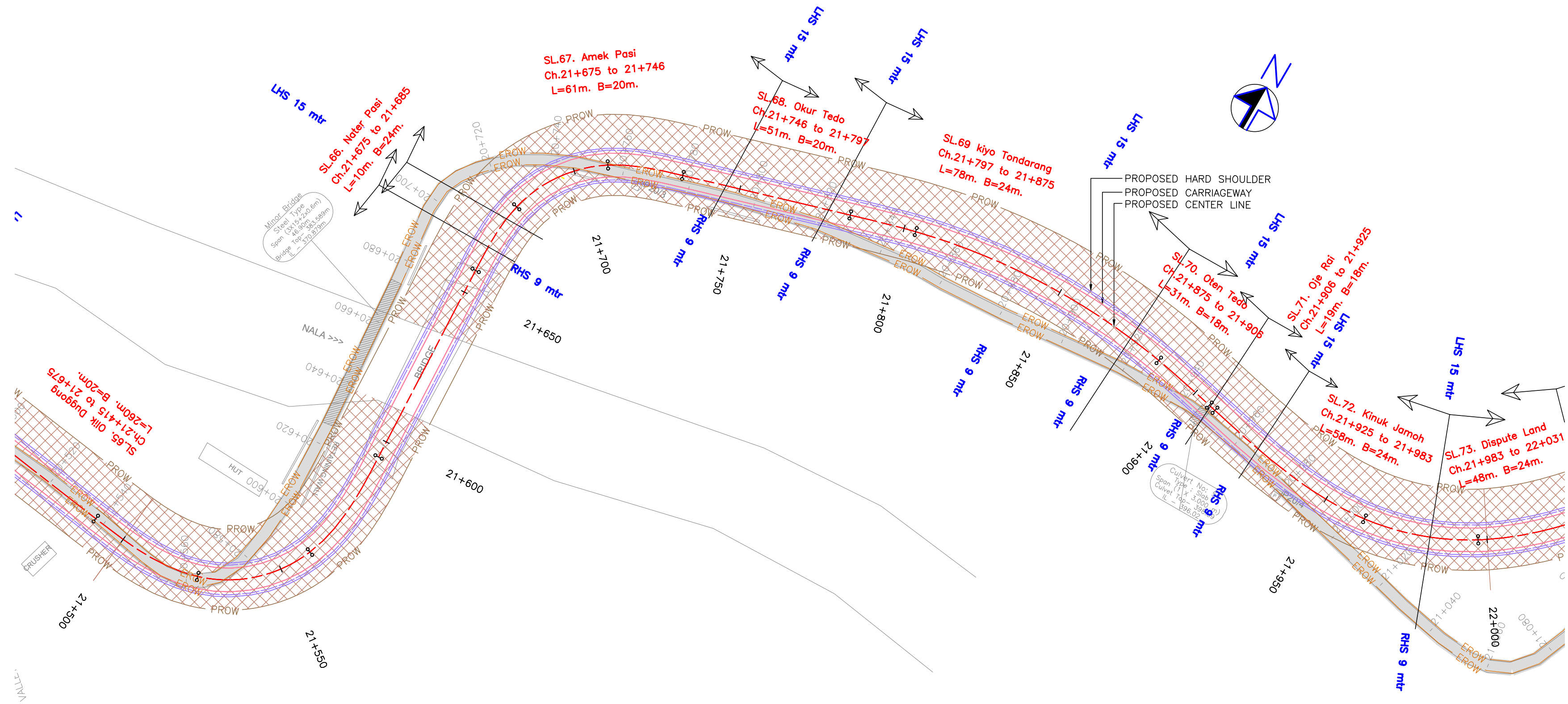
PLAN-KM 21+500 TO KM 22+000
