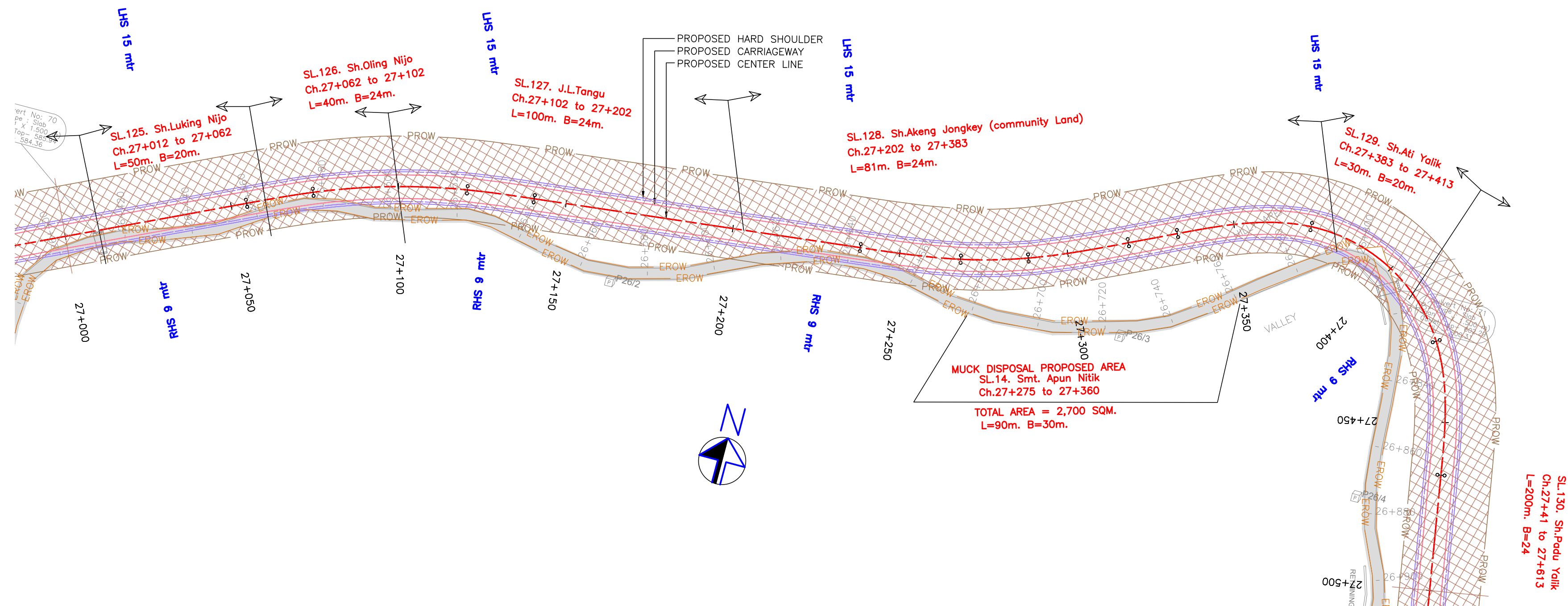
PLAN-KM 27+000 TO KM 27+500
