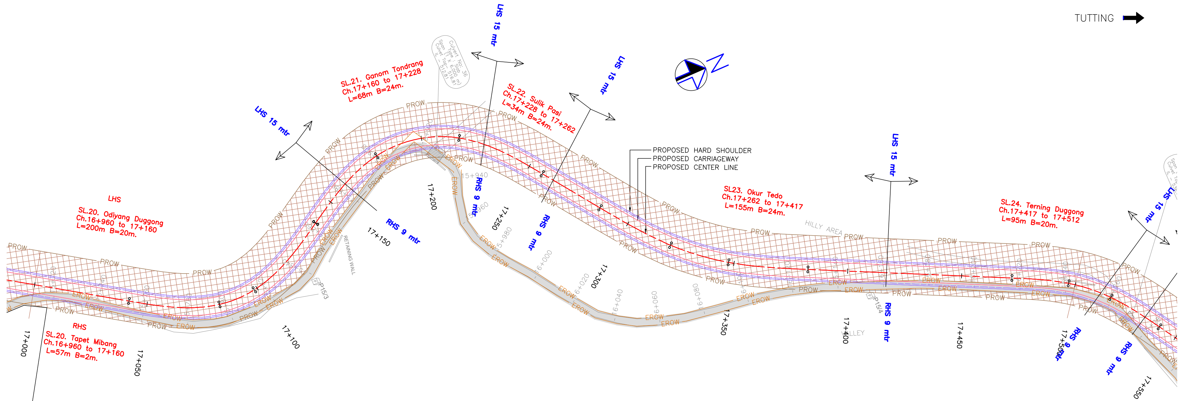
PLAN-KM 17+000 TO KM 17+500
