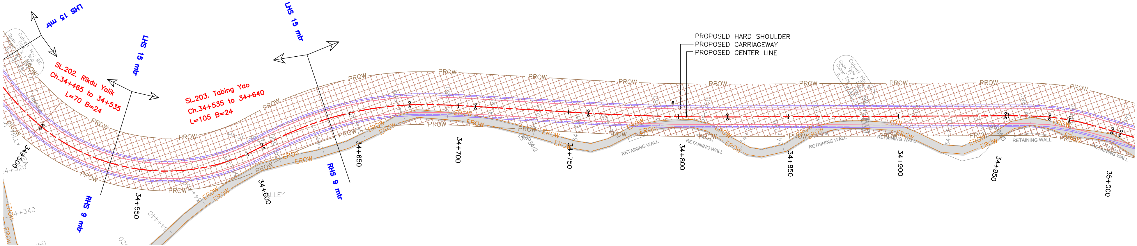
PLAN-KM 34+500 TO KM 35+000
