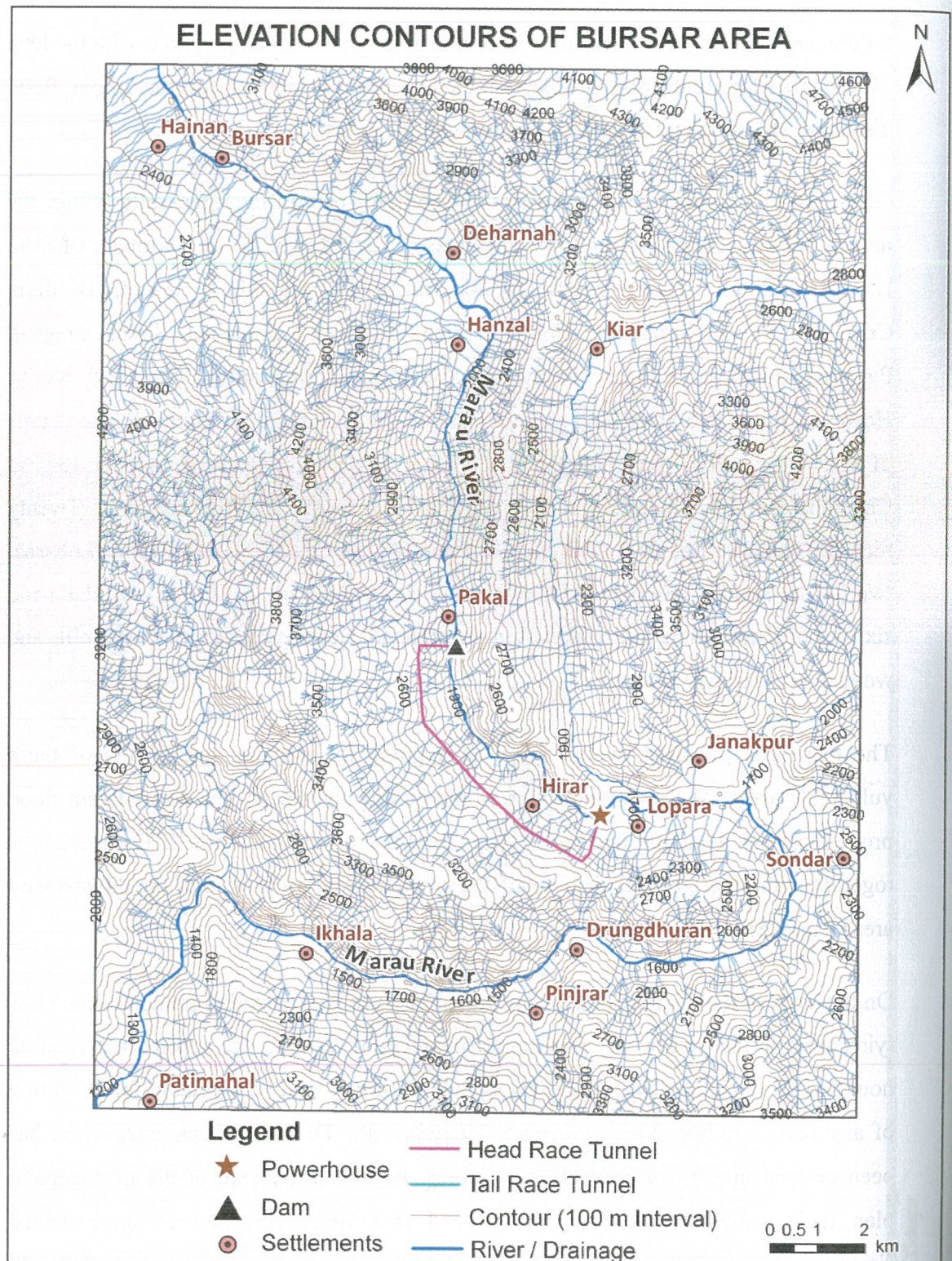
Fig. 9.5 Elevation contours of Bursar project area
