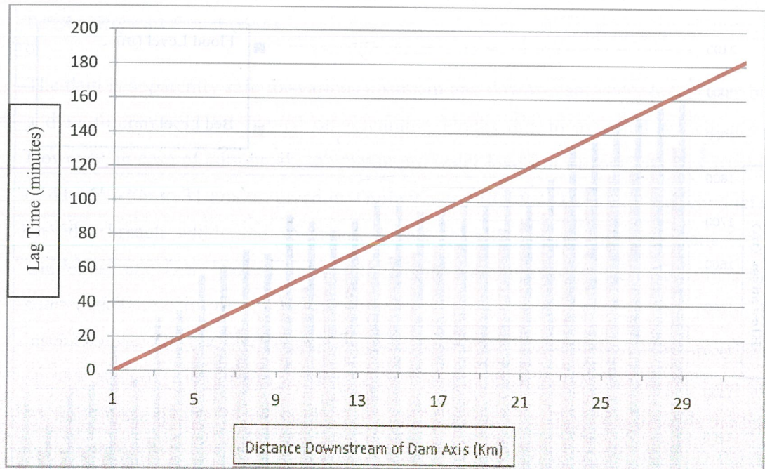
Fig. 9.3 (b) Time Lag Curve of Flood Wave
