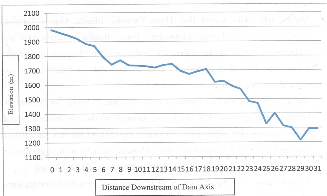
Fig. 9.3 (a) Flood Wave Level versus Different Downstream Locations
